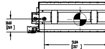
BOTTOM VIEW RSUB-415_A
