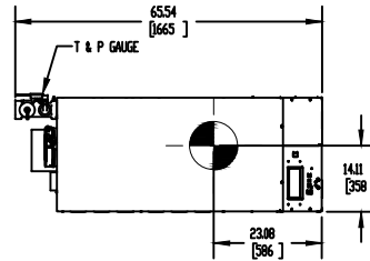
TOP VIEW RSUB-415_A
