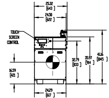
FRONT VIEW RSUB-415_A
